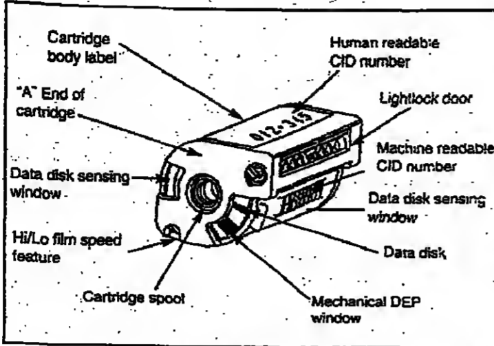
'A' end of APS 24 mm film cartridge which 'communicates' with the camera. (David Brauner)
